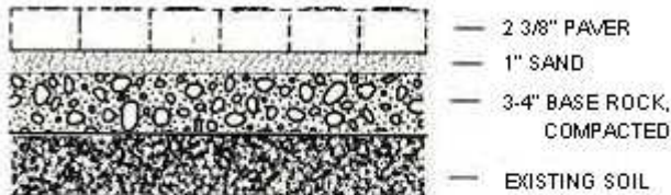
Cross Section Typical Installation for Patios and Sidewalks
